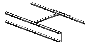
Kit for angle adjustable top includes cross brace and hinged front track
